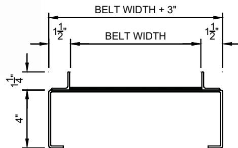
SECTION VIEW
