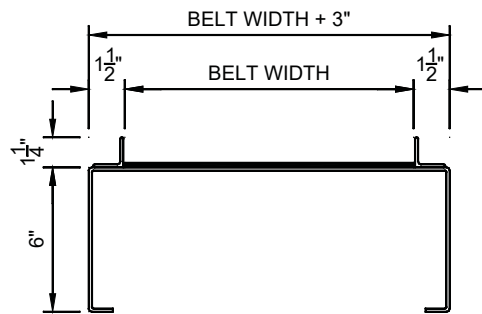
SECTION VIEW
