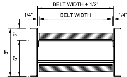
SECTION VIEW
