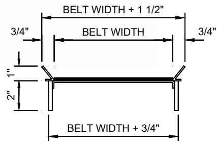
SECTION VIEW
