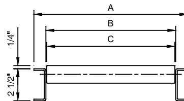
SECTION VIEW
