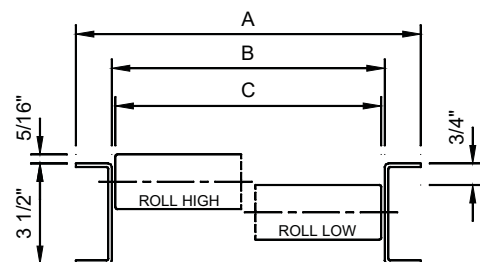
SECTION VIEW
