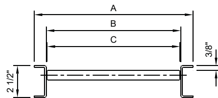
SECTION VIEW
