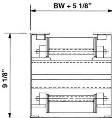
SECTION VIEW
