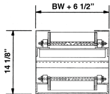
SECTION VIEW
