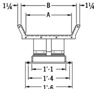
VIEW A-A WIDE BASE
