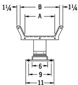
VIEW A-A NARROW BASE
